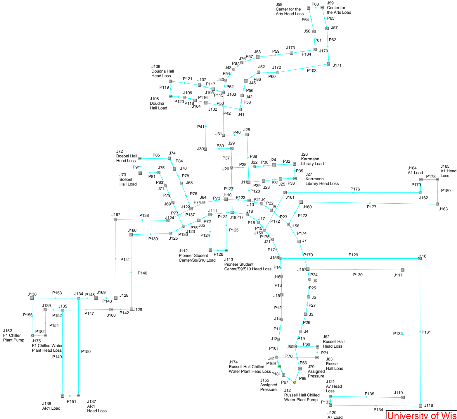
University of Wisconsin-Platteville Chilled Water Flow Analysis Phase 2 Campus
