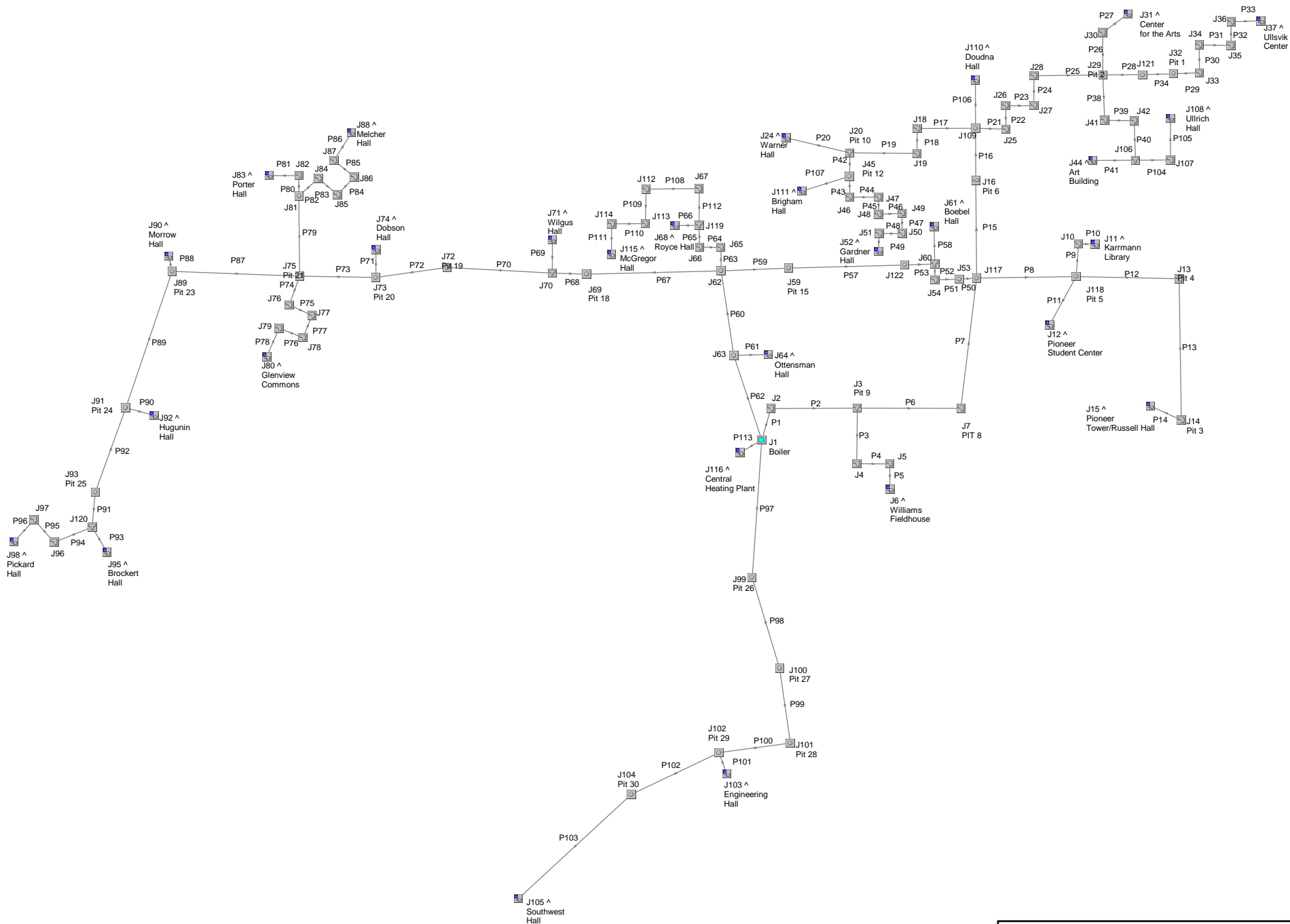
University of Wisconsin-Platteville Steam Flow Analysis Existing Campus
